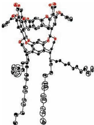
Figure 3. Crystal structure of 12 (displacement parameters are drawn to the 30% probability level).
