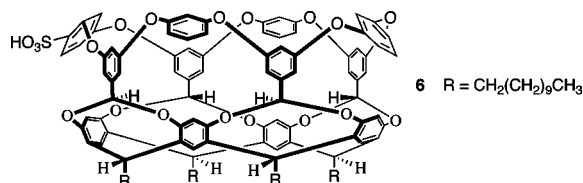
Figure 2. Chemical structure of 6 .
