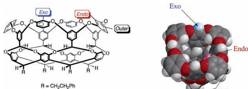
Figure 1. Chemical structure and space-filling model of cavitand 1 , showing the endo, exo, and outer positions.
